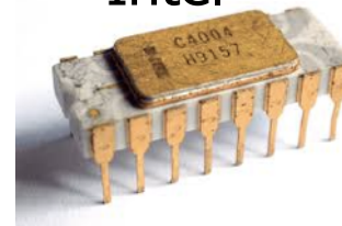
1968 Intel
