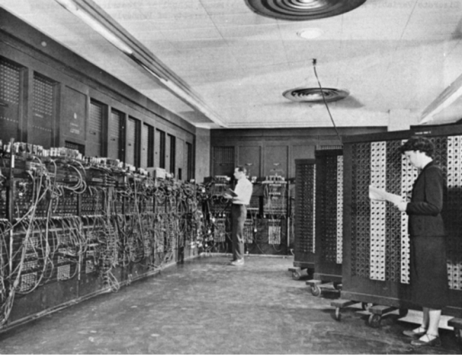
1944 Colossus, ENIAC
