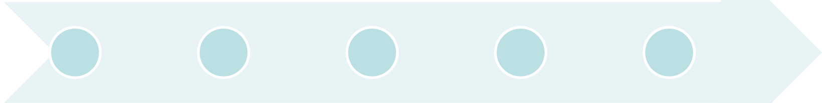
1951 UNIVAC
