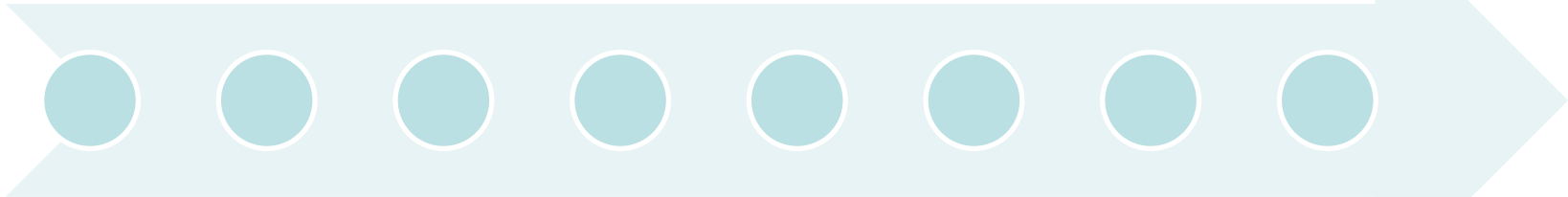
1997 Deep Blue
